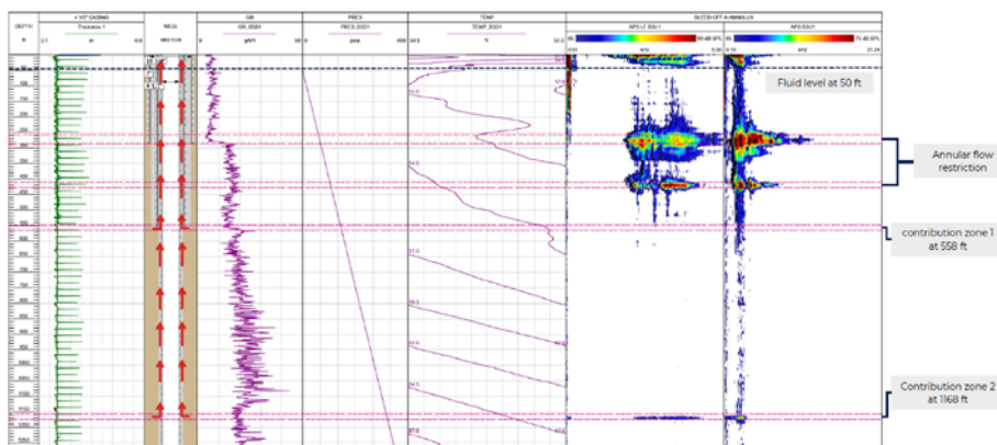
Noise-temp log indicating gas sources and obstructed flow.
